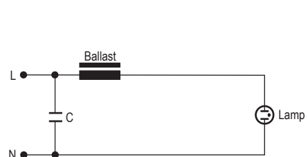
HID lamp circuit with parallel power factor correction capacitor.
