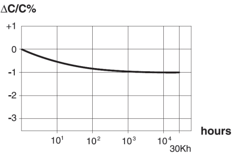
Capacitance versus Time under normal working conditions
