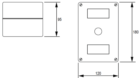
Enclosure type D490
