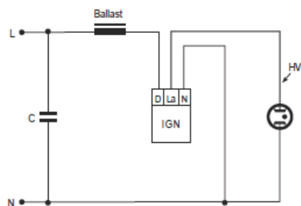
Superimposed-pulse ignitor circuit for LPS lamps
