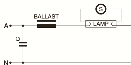
Switch start circuit
