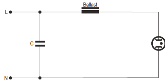
Single-voltage circuit for mercury vapour lamps
