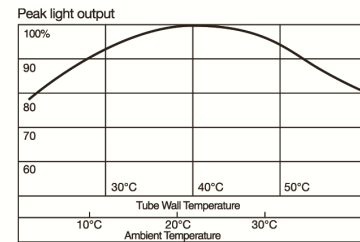
Typical relationship between temperature and lumen output
