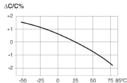
Capacitance versus Temperature
