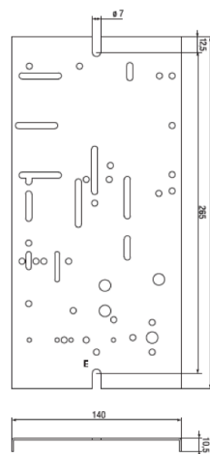
Gear tray to fit D430 box
