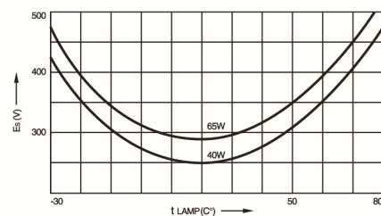
Start voltage versus ambient temperature
