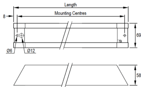
Enclosure type D427
