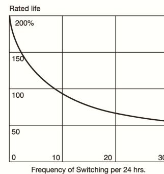
Typical effect on life of switching
