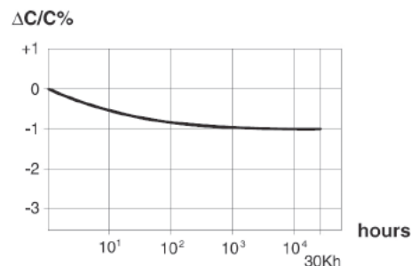
Capacitance versus Time under normal working conditions
