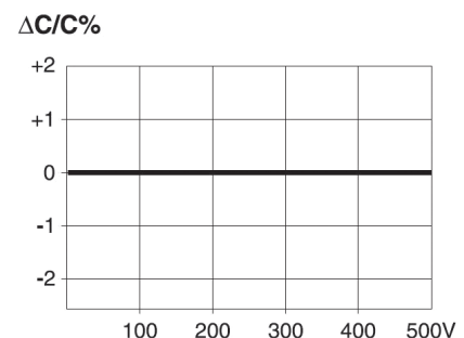
Capacitance versus Voltage
