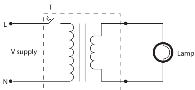
Low voltage lighting transformer circuit
