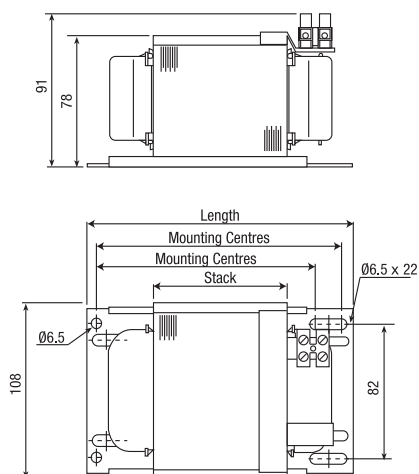
OG type ballasts with stack sizes 30–160 mm
