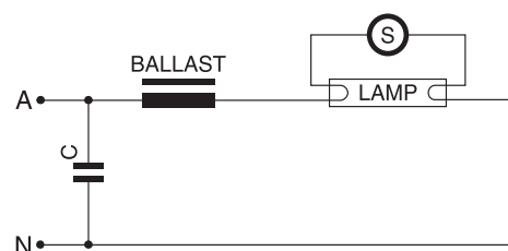
Switch start circuit
