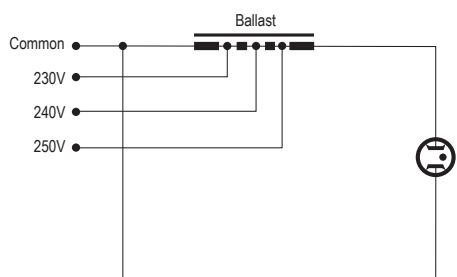
Leakage reactor ballast circuit for LPS lamps
