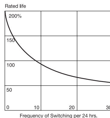
Typical effect on life of switching
