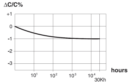
Capacitance versus Time under normal working conditions
