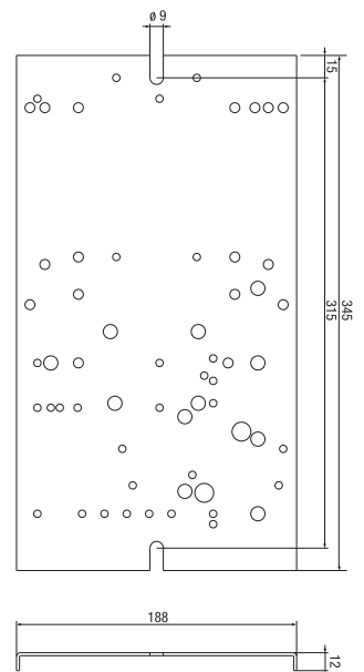
Gear tray for other applications
