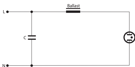
Single-voltage circuit for mercury vapour lamps
