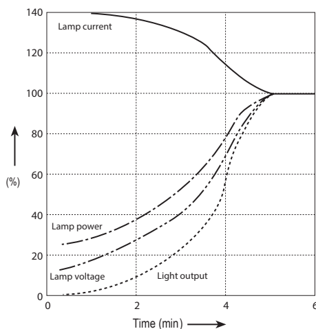
Unlike fluorescent lamps, mercury vapour lamps require several minutes to develop full light output as shown by these starting curves for a 400W mercury vapour lamp
