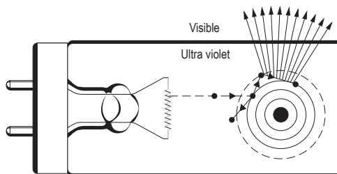
De-activation of excited mercury atoms produce UV photon and is converted to visible light by the internal phosphor coating of the fluorescent lamp.
