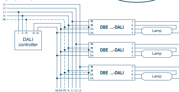
Sample DALI wiring diagram:
