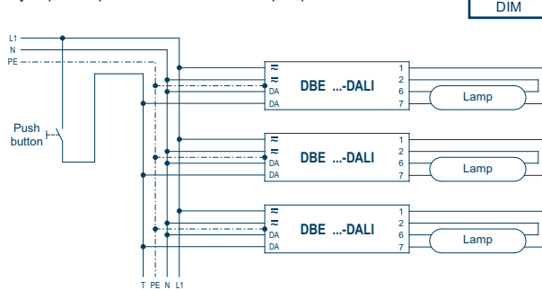
Sample Touch DIM wiring diagram:
