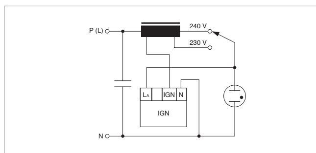
Multi-voltage circuit with pulse ignitors for sodium vapour lamps and metal halide lamps
