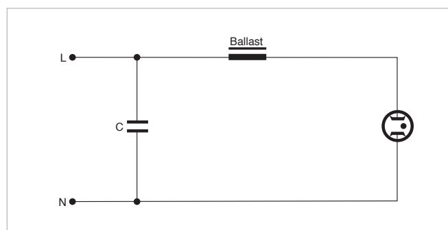
Single-voltage circuit for mercury vapour lamps
