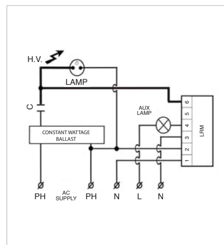
C) Constant wattage type circuit (3 phase)
